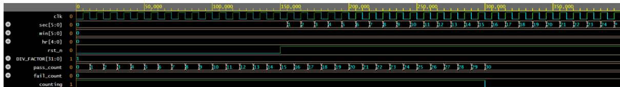
Figure 3: Waveform for reset_test
